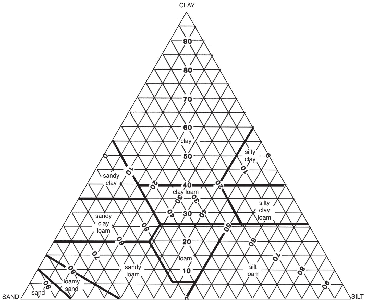
Figure 8.—Official textural triangle. The scales of sand, silt, and clay, along with the precise boundaries between soil textural classes, are used to determine the correct name for the texture of a soil sample.
